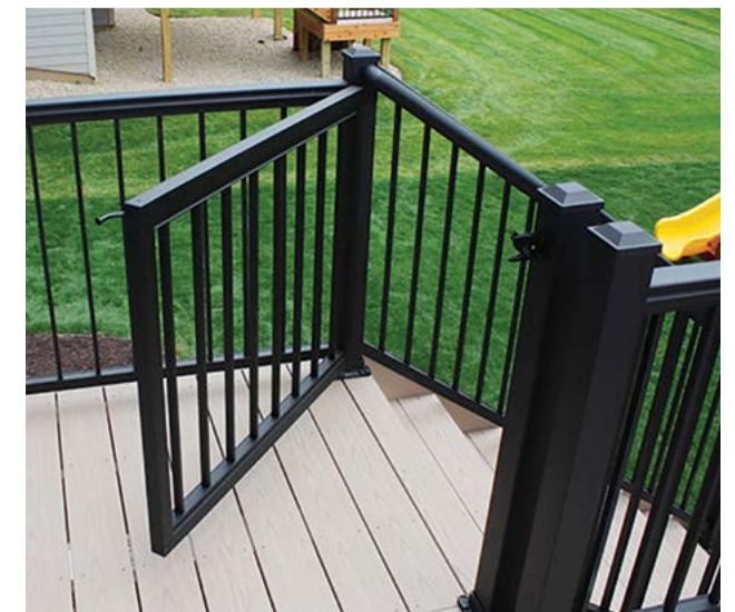
IMPRESSION RAIL EXPRESS GATE KIT An aluminum rail kit used for 36" or 42" rail heights. Available in White, Black, or Dark Bronze.
