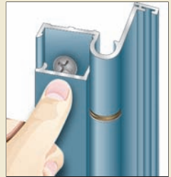
Colors Matched Aluminum Screw Cover
